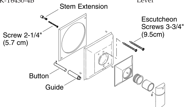
Deep Rough-In Kit Parts
