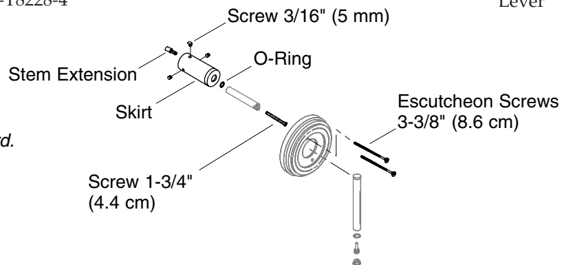
Deep Rough-In Kit Parts
