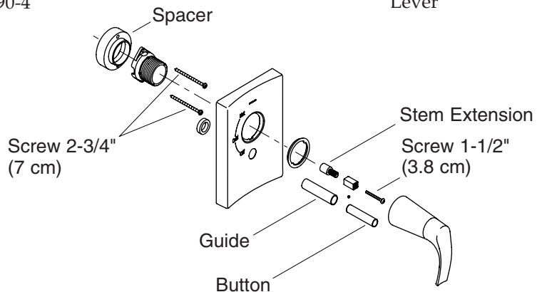
Deep Rough-In Kit Parts
