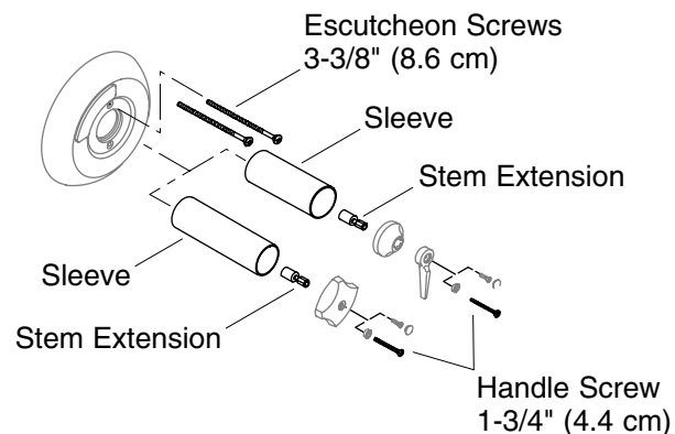
Deep Rough-In Kit Parts
