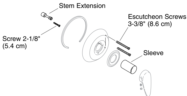
Deep Rough-In Kit Parts
