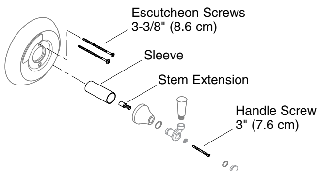
Deep Rough-In Kit Parts
