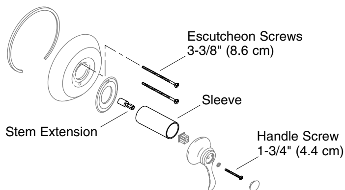
Deep Rough-In Kit Parts
