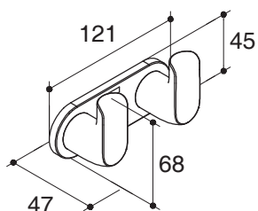
K-97500T
