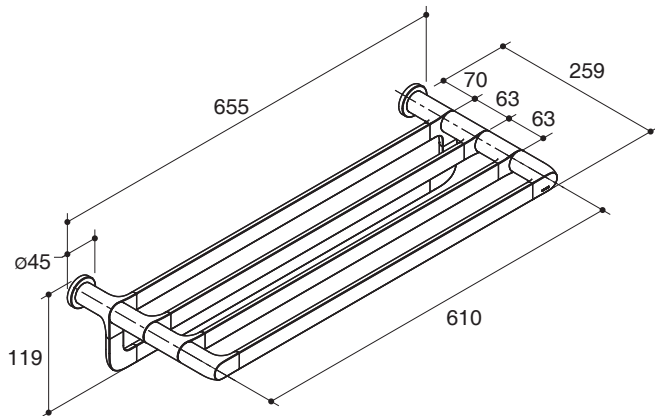
K-97497X, K-97497T
