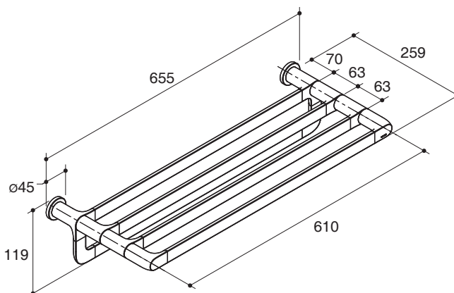
K-97497X, K-97497T
