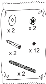
1223187 Mounting Kit
