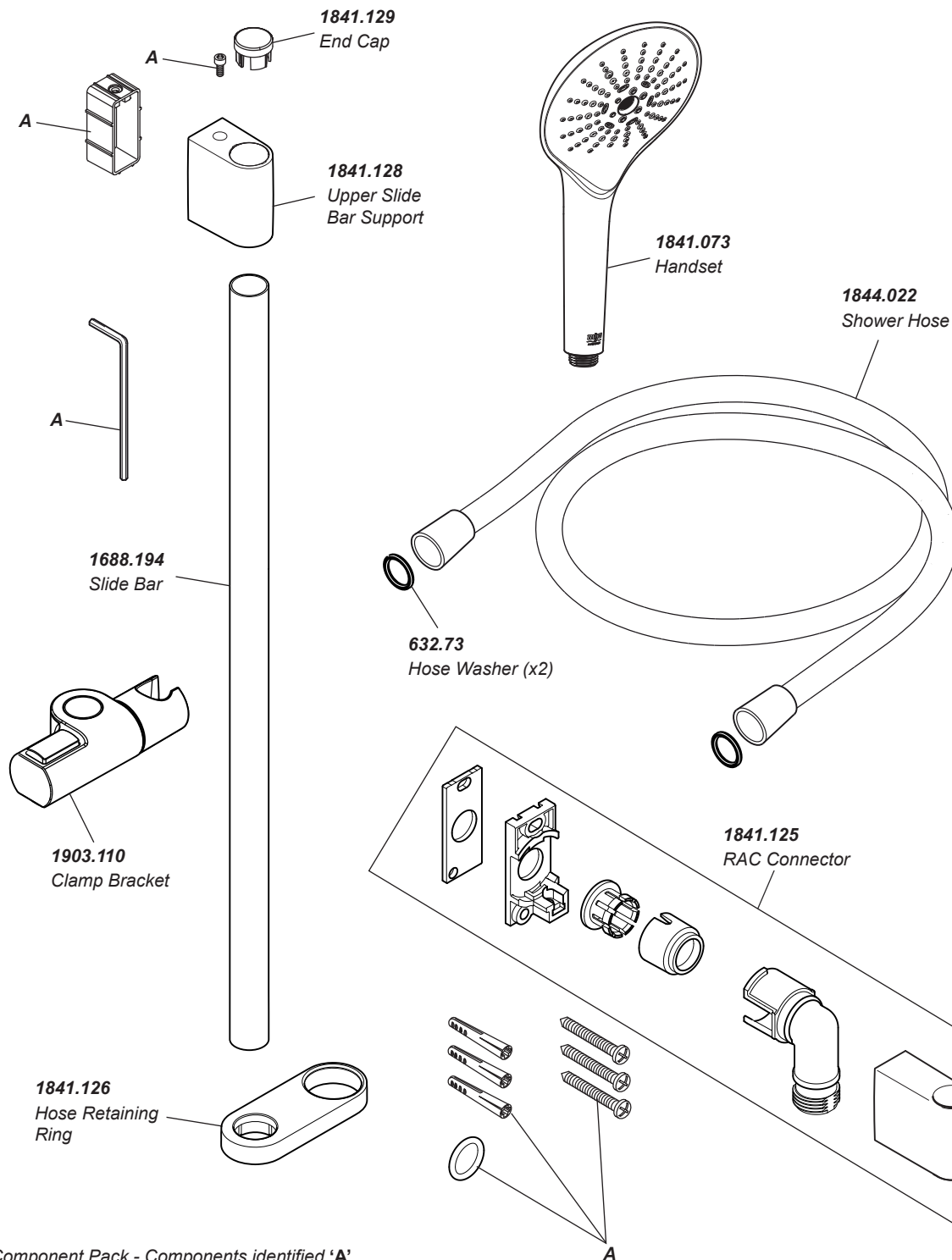
1841.130 Component Pack - Components identified 'A'
