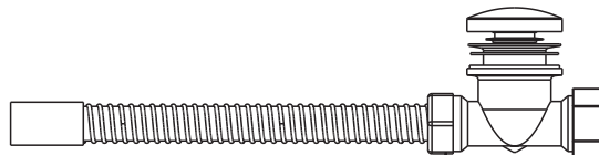
This nut is removable to change the direct of drain pipe is nessory. 如有需要，可拆卸螺母以变换排水软管方向。 Ensure no leakage after change the pipe direct. 更换排水软管方向后，请再次确认连接处未漏水。
