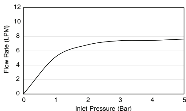
Flow Curve
