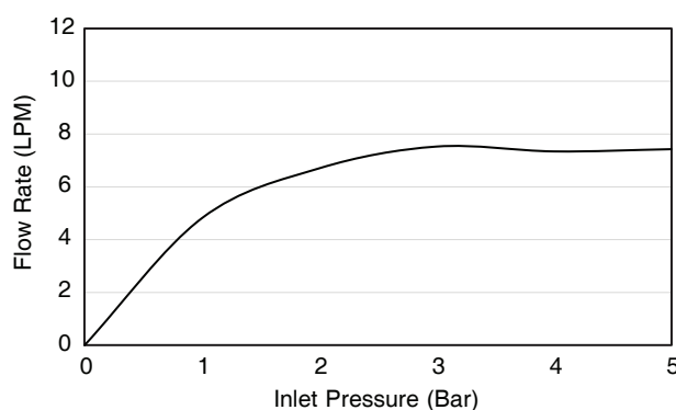
Flow Curve
