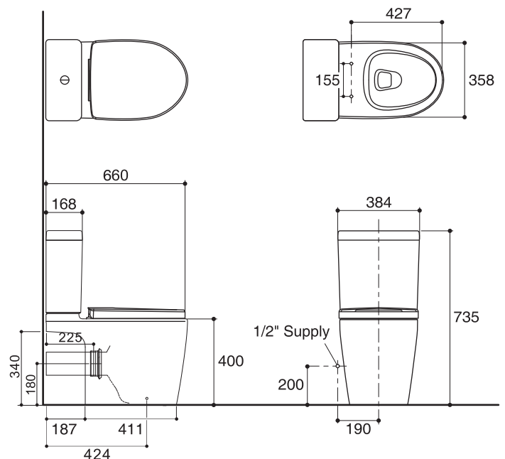
Wall Discharge
