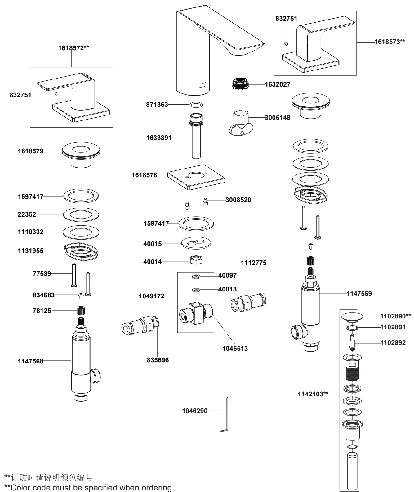
EX38214T-4 8寸脸盆龙头
