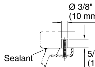
Marble Installation
