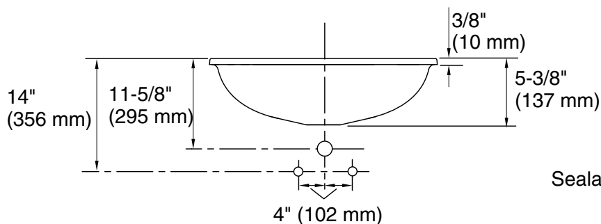
Standard Installation
