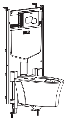
In-Wall Tank With Frame 入墙式隐藏水箱（含固定支架）坐便器
