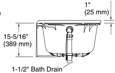
Integral Flange Detail
