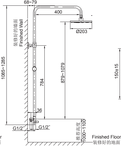
72678T-B7
