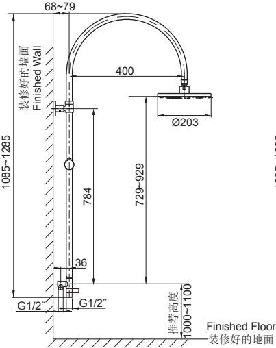
72676T-B7
