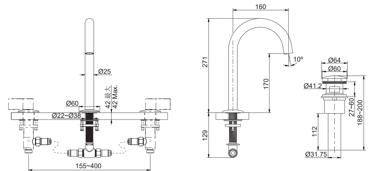
77967T/77967T-MU
