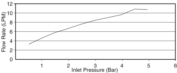
Flow Curve
