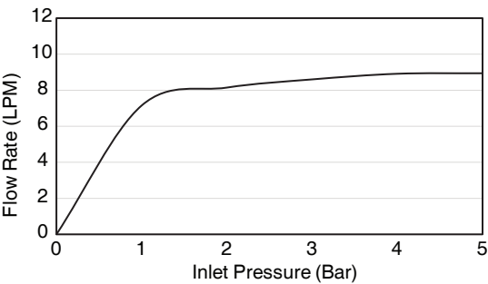
Flow Curve (K-98951T-L)
