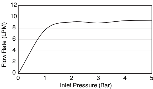
Flow Curve (K-98952T-L)
