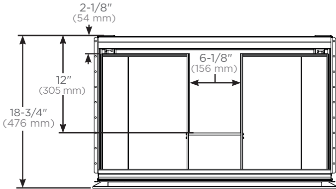
Top view for plumbing and sink clearance
