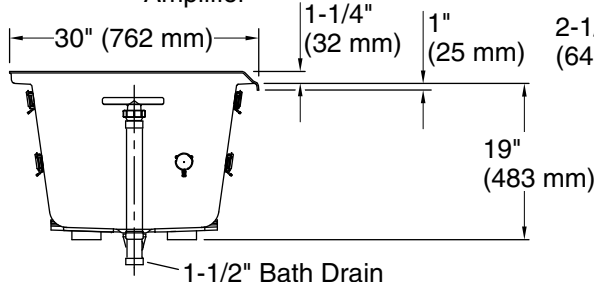
Amplifier
