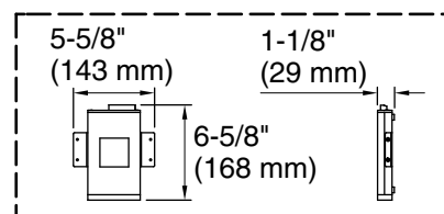
Amplifier
