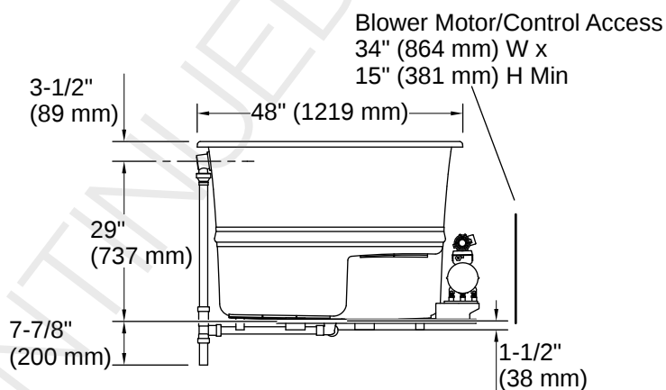
Drop-in Rim Detail
