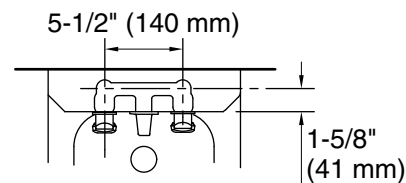
Faucet Detail
