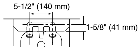
Faucet Detail
