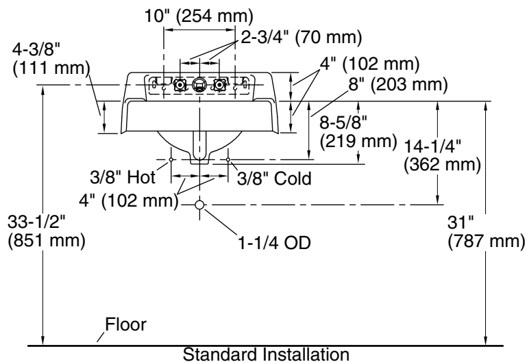
Standard Installation
