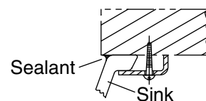
Wood Counter Installation
