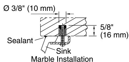
Recommended ADA Installation
