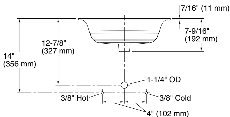
Standard Installation
