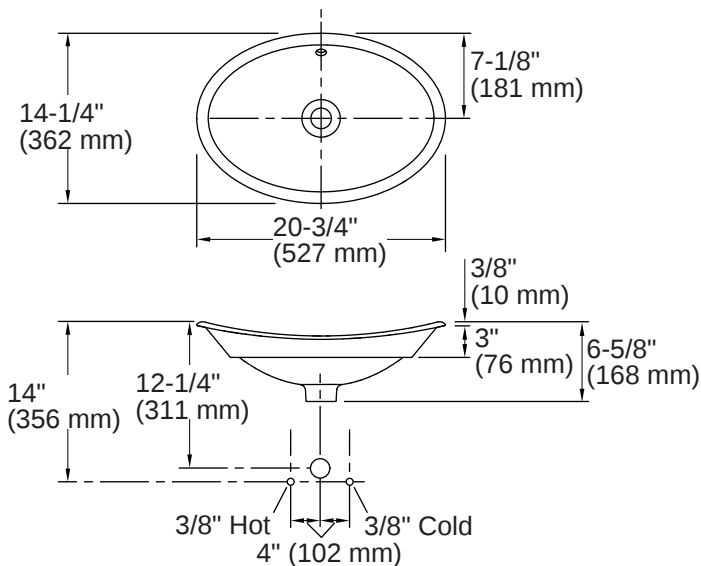
Standard Installation
