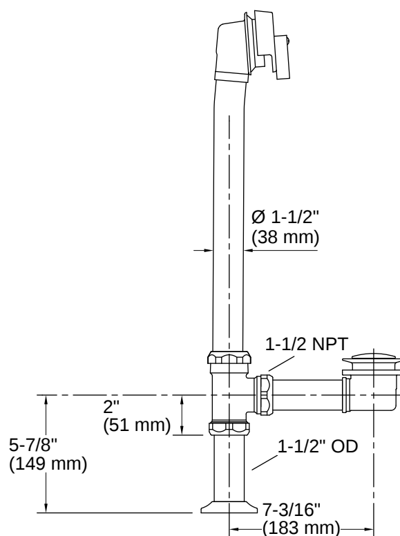
Through-the-Floor
