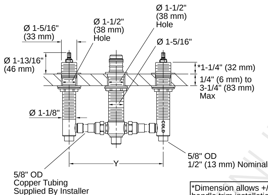
Finished Deck-Mount Installation
