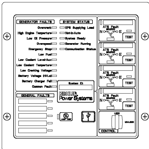
RSA III with Four ATS Controls
